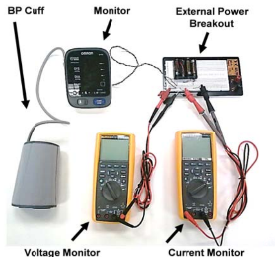
Figure 5: The automatic Omron Ten Series Blood Pressure Measurement Device prepared for voltage and current measurements. Voltage and current are monitored using two multimeters.
